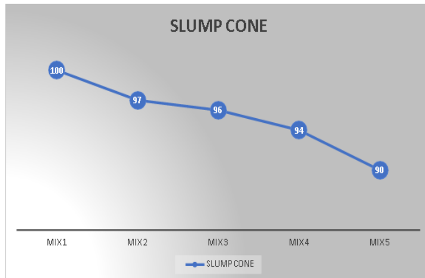
Graph 5.1 slump cone test results
