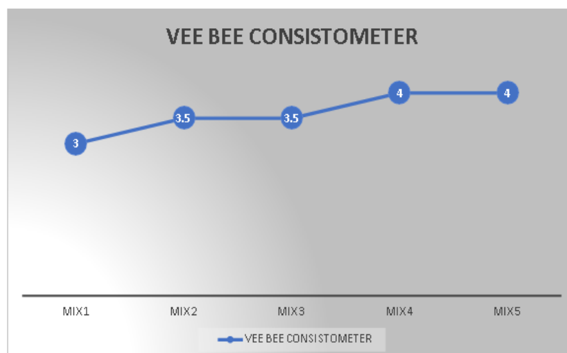
Graph 5.3. vee bee consistometer test results.
